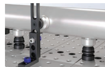
Vertical application using Locating Post + V-Block Spacer
